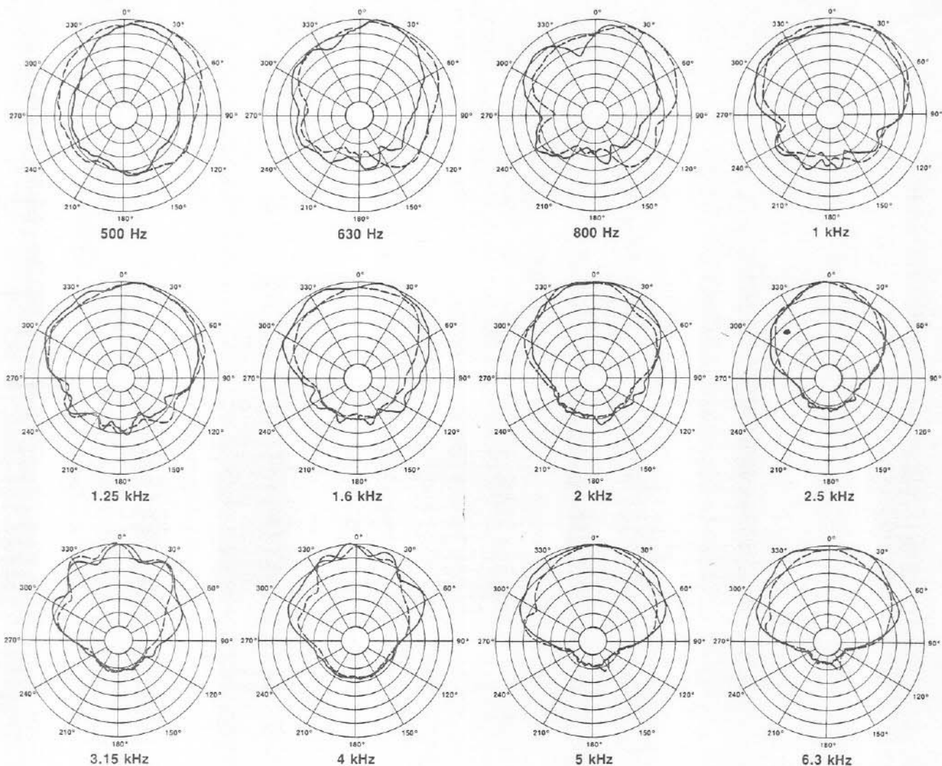
FIGURE 1 PI 15-3 Polar Response
