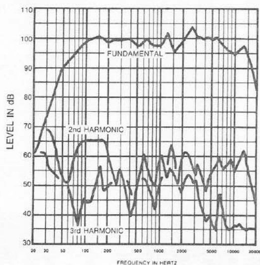
FIGURE 3 PI 15-3 Frequency Response (1 watt at 1 meter)
